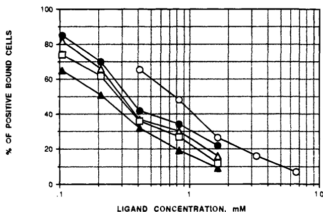
Figure 3. Inhibition of HL-60 adhesion to recombinant soluble E-selectin-coated plates: (O) pentasaccharide, NeuAc \alpha 2,3-Gal \beta 1,4-(Fuc \alpha 1,3-)GlcNAc \beta 1,4-Gal \beta OEt; (▲) 3,6-dimer 6 ; (△) 4,6-dimer 16 ; (●) 2,6-dimer 17 ; (□) 2,3-dimer 18 . Compounds 29 and 33 exhibited similar activities as the pentasaccharide.
