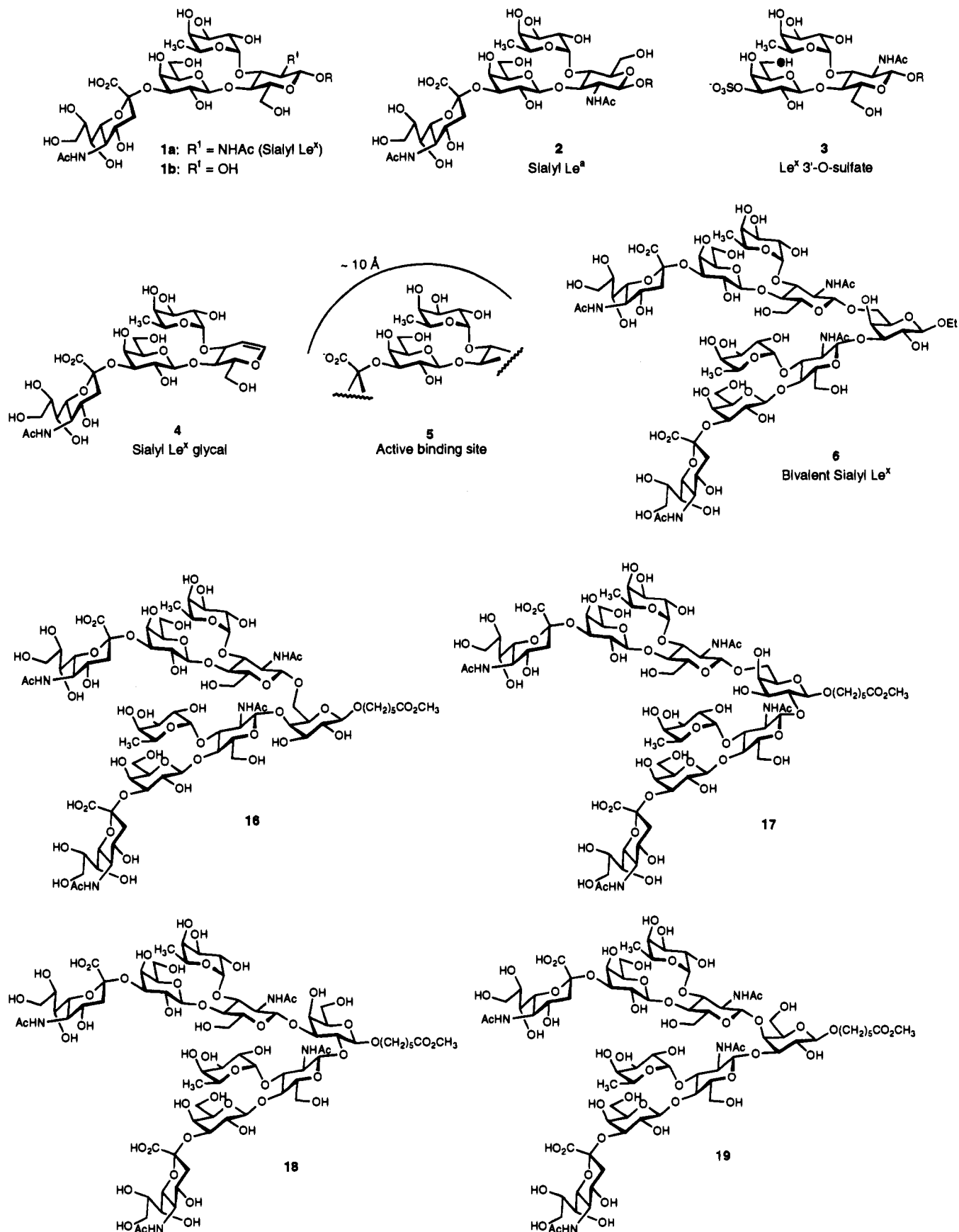
Figure 2. Ligands for E-selectin (1-6) and (b) Sialyl Lewis x dimers (16-19).
