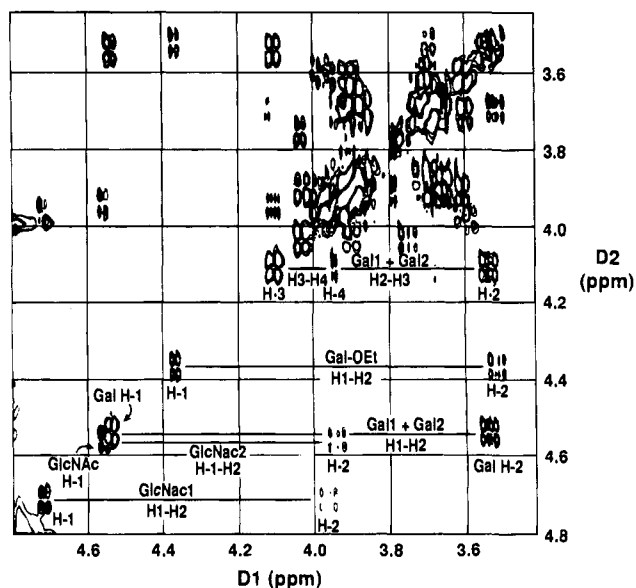
Figure 4. (Top) 2D phase-sensitive double quantum filter COSY (COSYDFPT) of 6 . (Bottom) expansion of 2D COSYDFPT of 6 .
